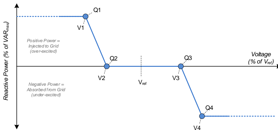
Figure 25 - Volt/VAR Configuration
