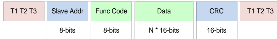
Figure 32 - RTU Message Frame (PDU) Format
