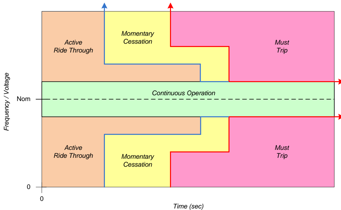
Figure 27 - Ride Through Cessation and Trip Curves
