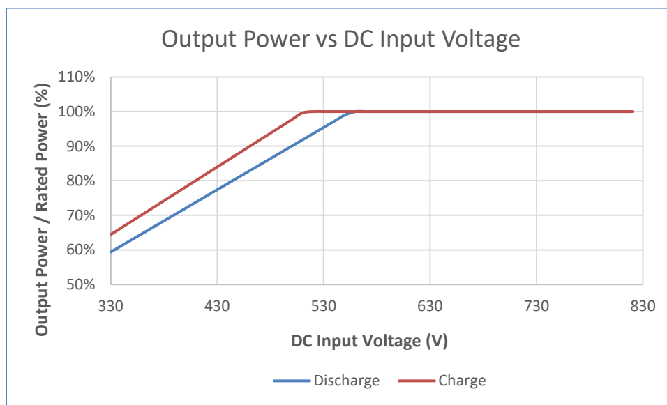
Figure 8 - DC Input Voltage Derating Curve
