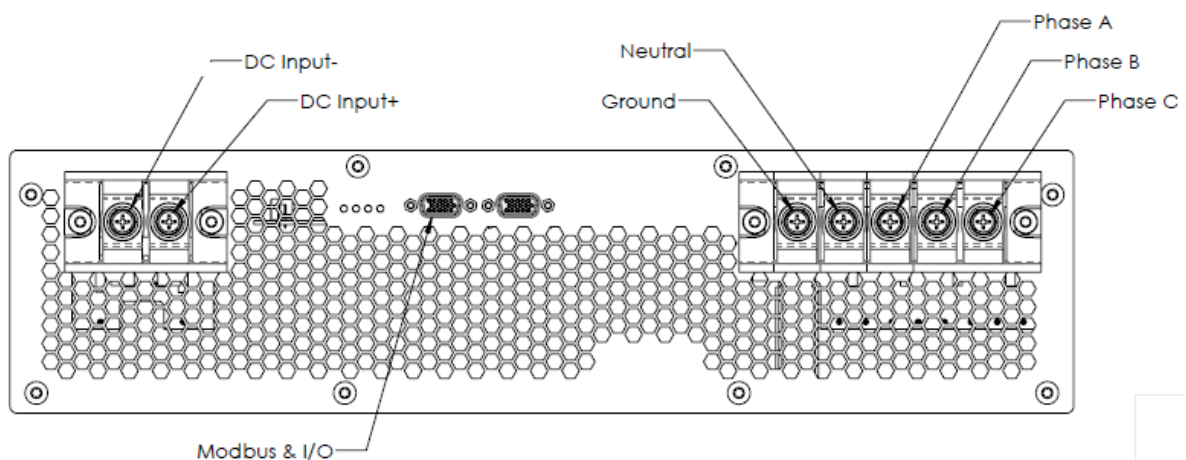
Figure 13 - Interface Identification and Location
