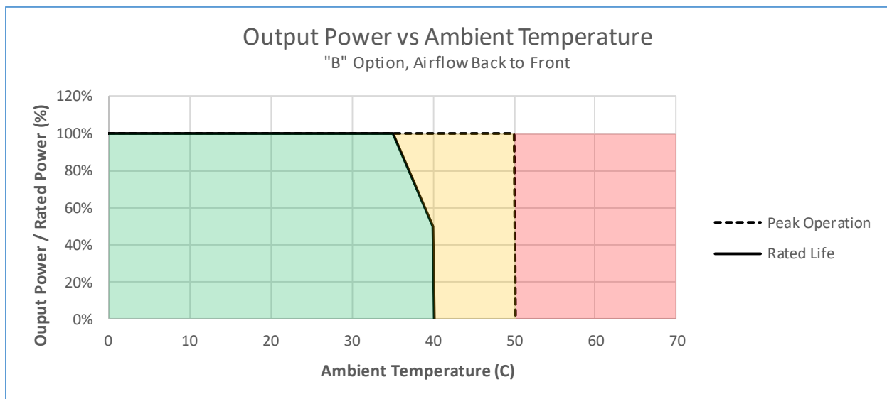
Figure 7 - Temperature Derating Curve – “B” Option
