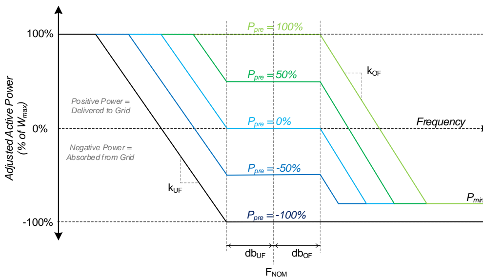
Figure 24 - Frequency/Watt Configuration
