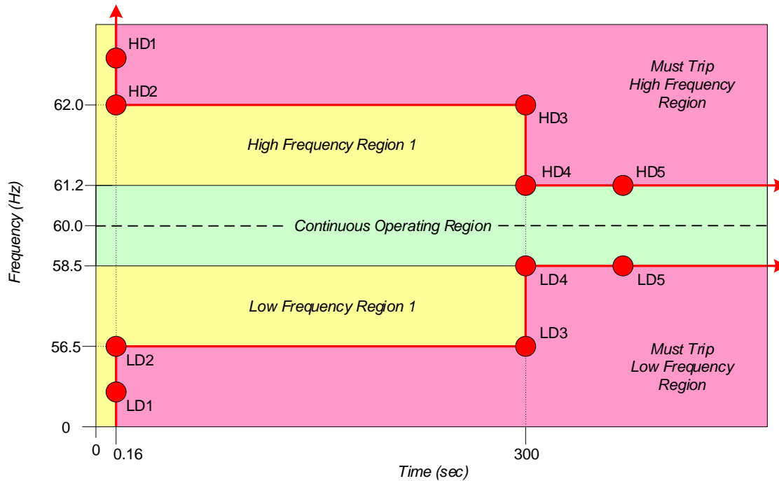
Figure 29 - Frequency Ride Through IEEE 1547-2018 Configuration
