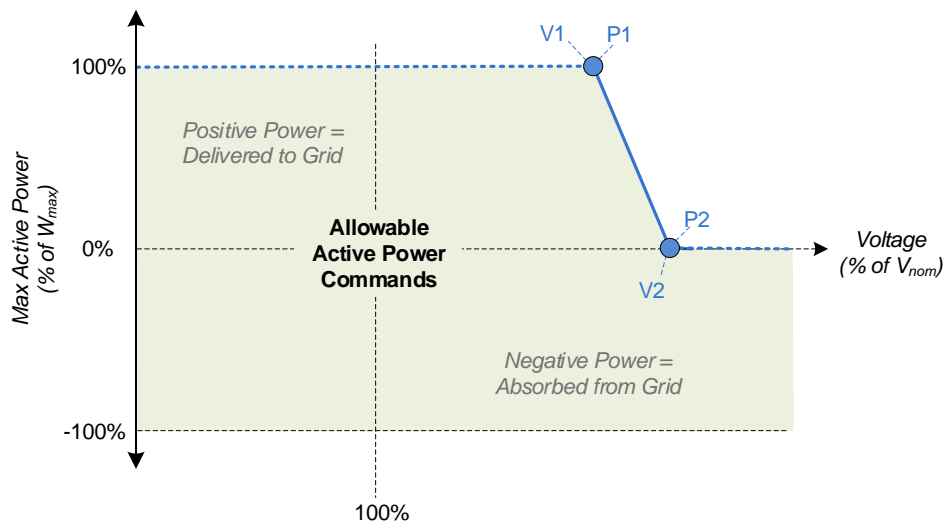
Figure 23 - Volt/Watt Configuration
