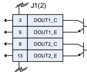
Figure 20 - Discrete Output Interface
