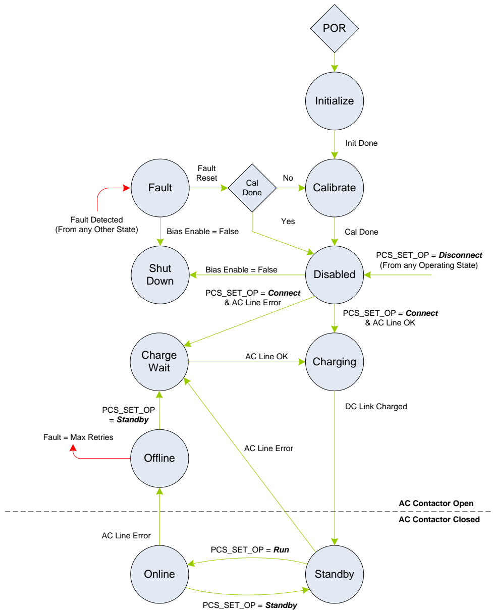
Figure 21 - State Machine
